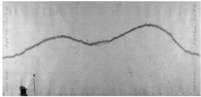
Figure 4. Marigram from 5 March 1862, from San Francisco, California. Nontidal fluctuations are evident and required interpolation by the tabulator to estimate the astronomical low water (see interpolation line and low-water point). The thick pencil line indicates atypical, short (<1 minute) fluctuations caused by a stilling well problem or by dock vibrations after moving the gauge to a new gauge house, which was necessitated by the severe storms of December 1861 to February 1862.
